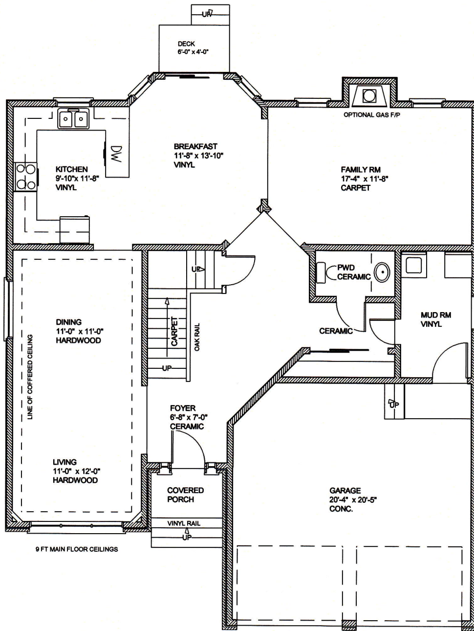
THE ARLINGTON GROUND FLOOR PLAN
